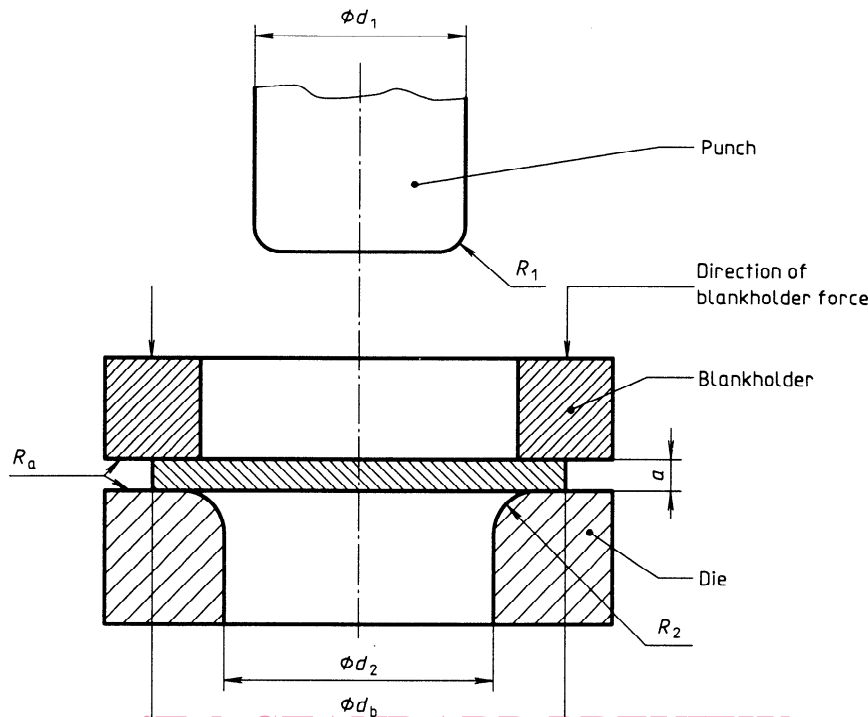
Figure 2 — Schematic diagram of test equipment
