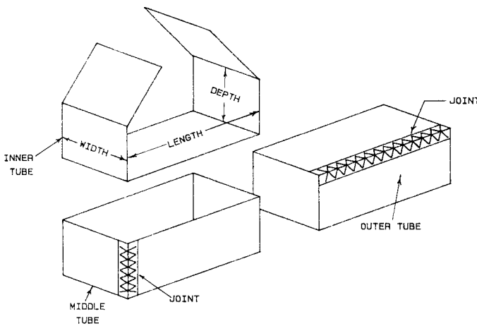
FIG. 13 Box, Fiberboard; TS—Triple Slide Box
