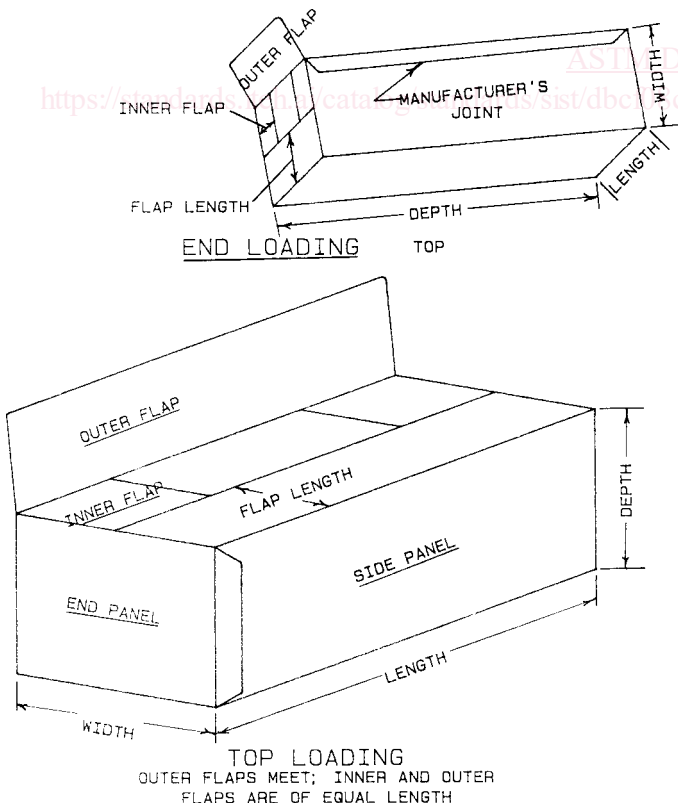
FIG. 1 Box, Fiberboard; RSC—Regular Slotted Box
