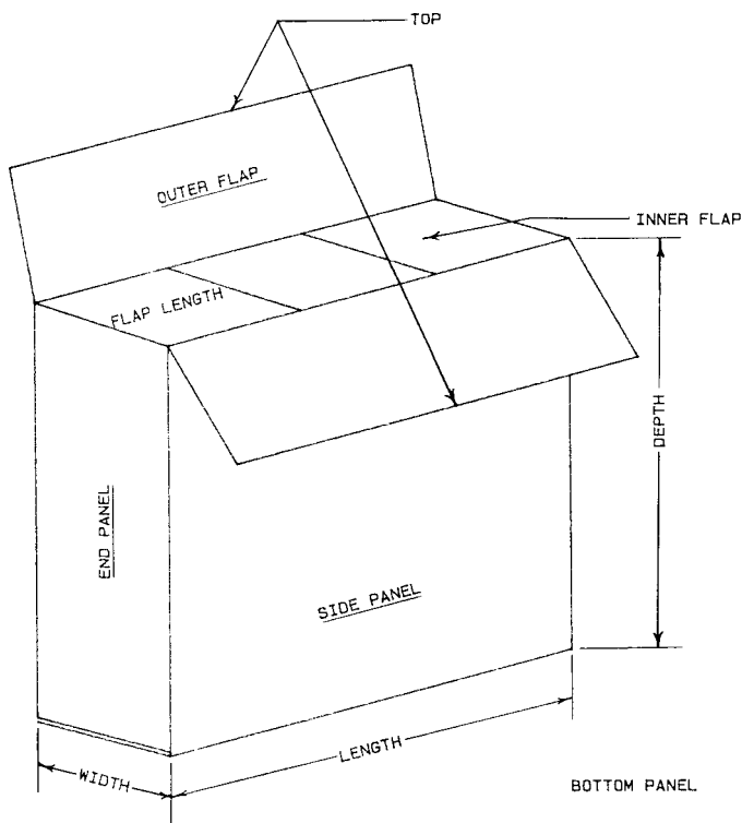
FIG. 3 Box, Fiberboard; FOL—Full Overlap Slotted Box
