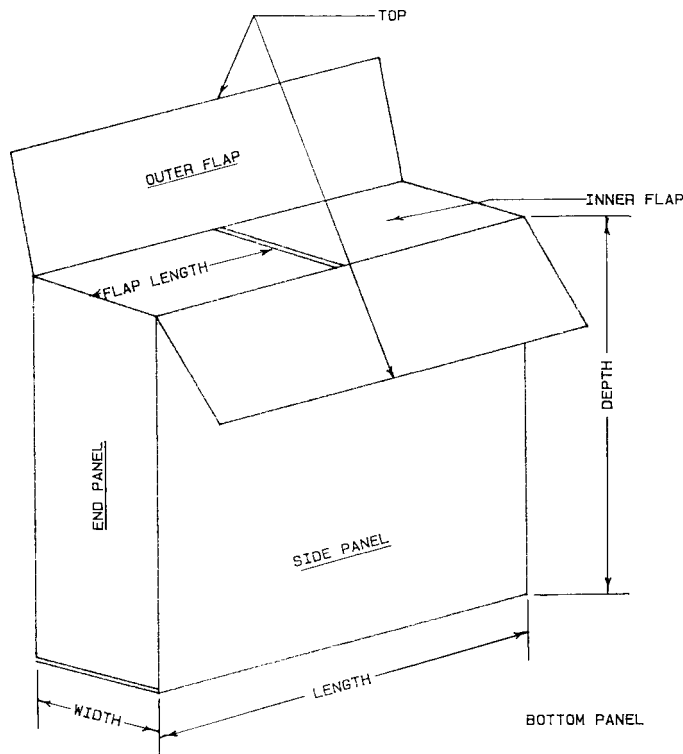
FIG. 4 Box, Fiberboard; SFF—Special Full Flap Slotted Box
