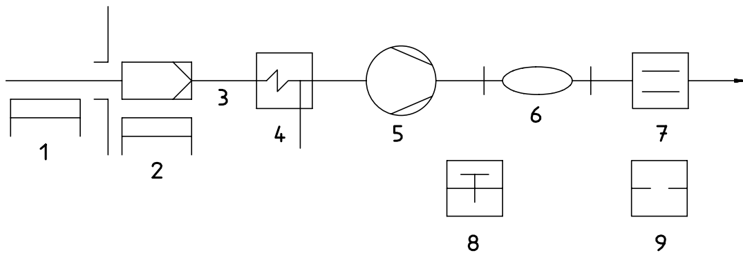
a) Heated sampling system, sampling flask with two taps https://standards.iteh.ai/catalog/standards/sist/6428a29d-6e66-4721-a17b-d298a00f3942/iso-11564-1998
