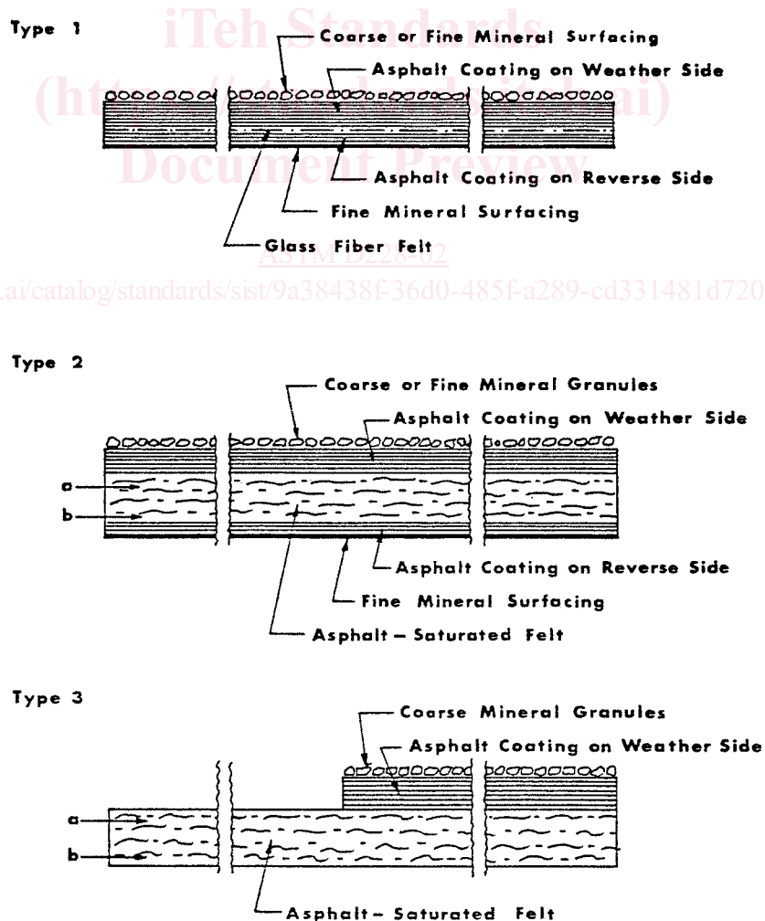
FIG. 1 Types of Asphalt-Coated Roll Roofing and Shingles
