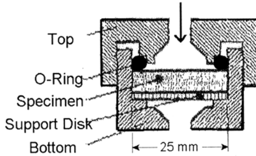
FIG. 1 Closed Filter Holder
