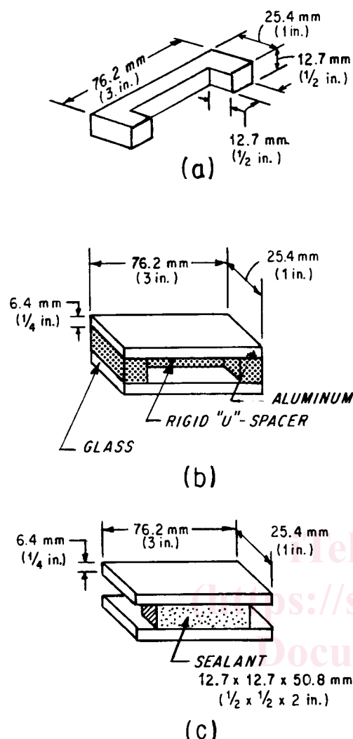
FIG. 1 Preparation of Test Specimen
