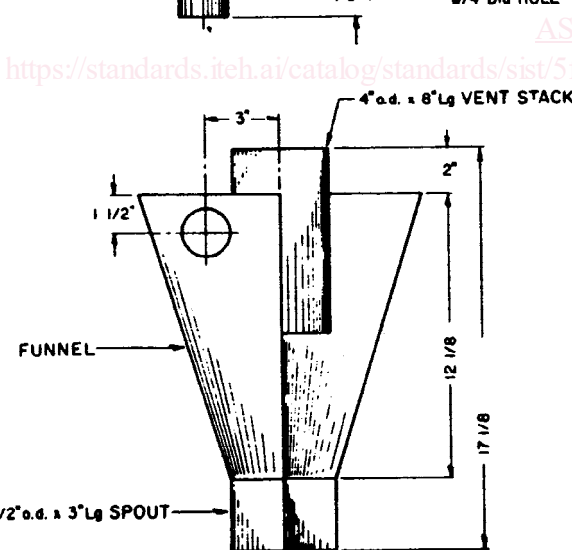
FIG. 2 Cyclone Receiver Weldment
