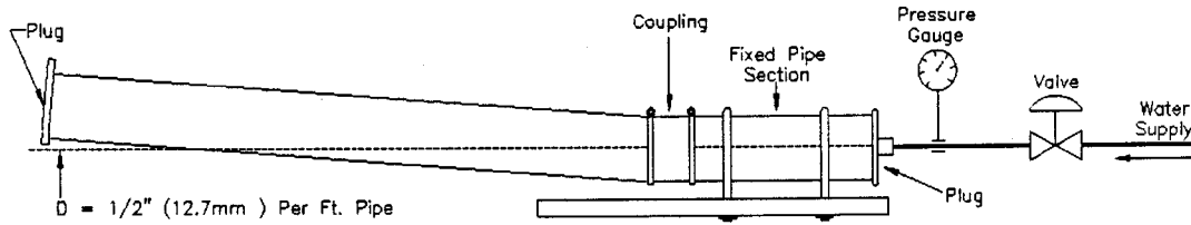
FIG. 1 Deflection Test
