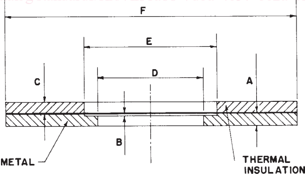
FIG. 1 Cleveland Open Cup Apparatus
