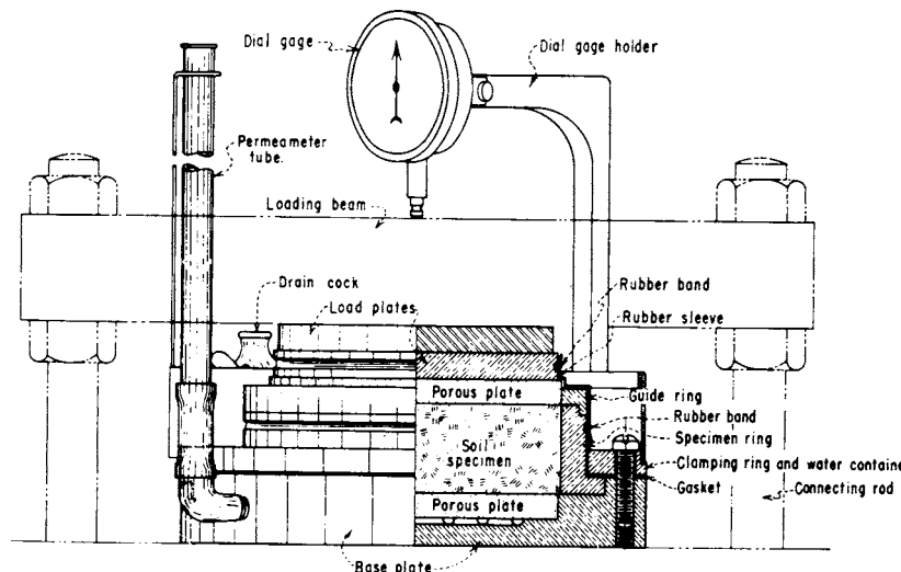
FIG. 1 Fixed-Ring Consolidometer
