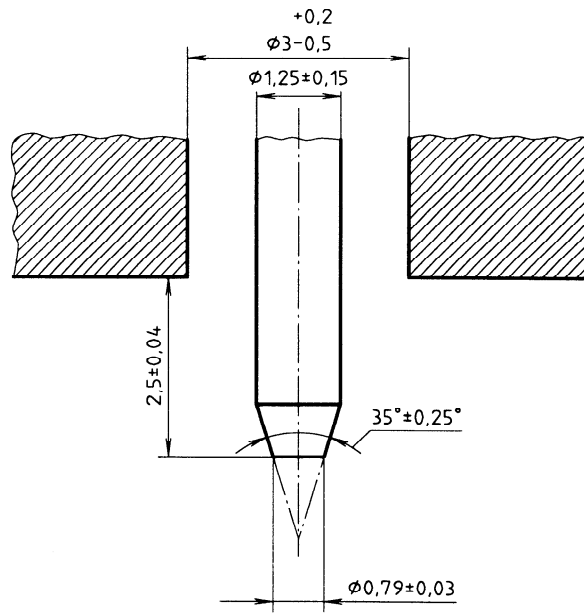
Figure 1 — Indentor for type A durometer (standards.iteh.ai)
