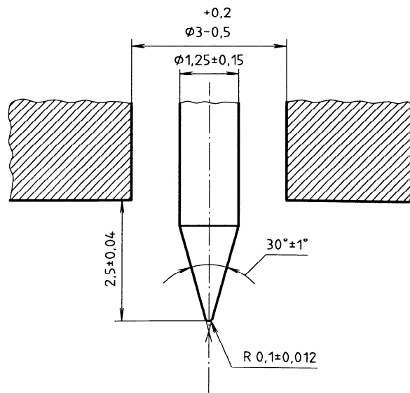
Figure 2 — Indentor for type D durometer
