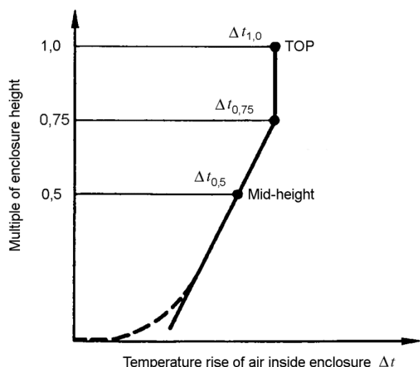
Figure 2 – Temperature-rise characteristic curve for enclosures with A_e not exceeding 1,25 m 2
