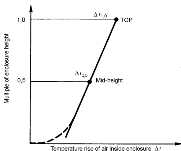
Figure 1 – Temperature-rise characteristic curve for enclosures with A_e exceeding 1,25 m 2
