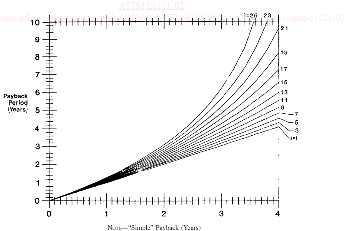
FIG. 1 Graphical Solution to Payback Period: SPB = 0 to 4 Years, i = 1 to 25 % (odd)
