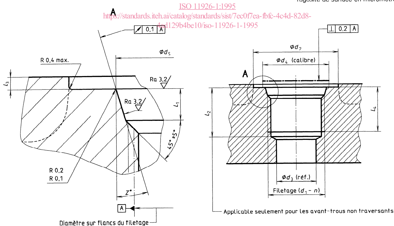
Figure 1 — Orifice
