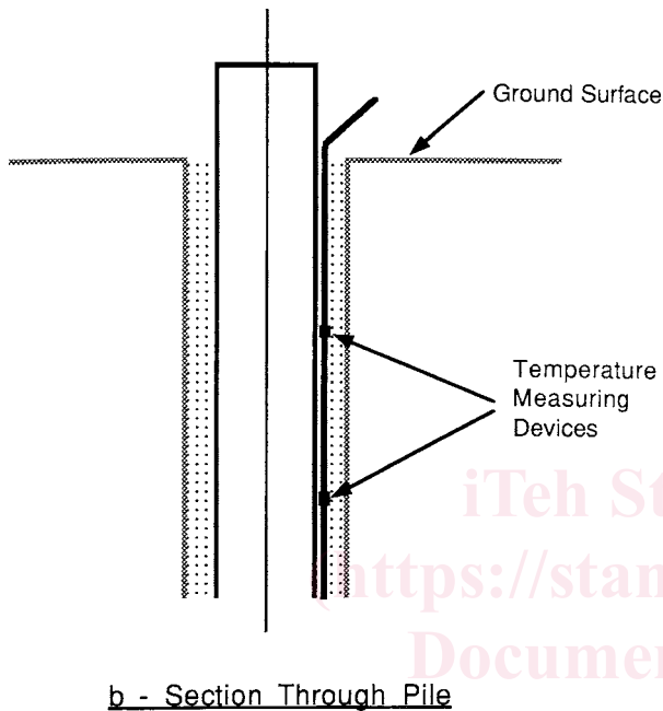
FIG. 1 Placement of Temperature Measuring Devices for Slurried Test Pile
