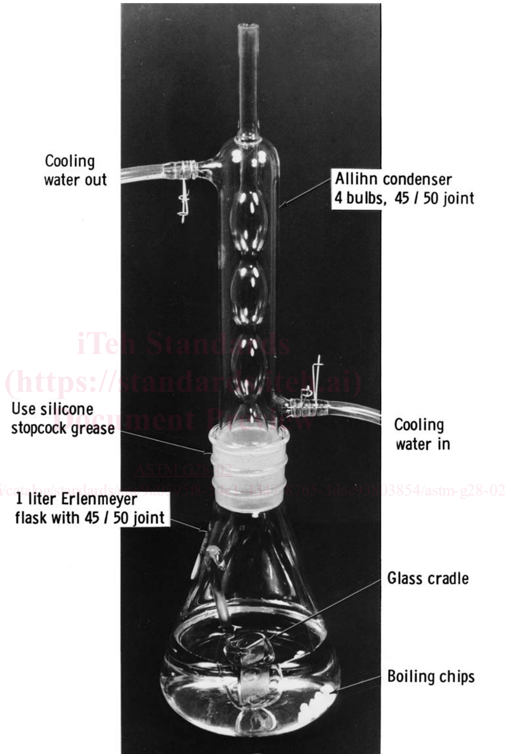
FIG. 1 Apparatus for Ferric Sulfate-Sulfuric Acid Test
