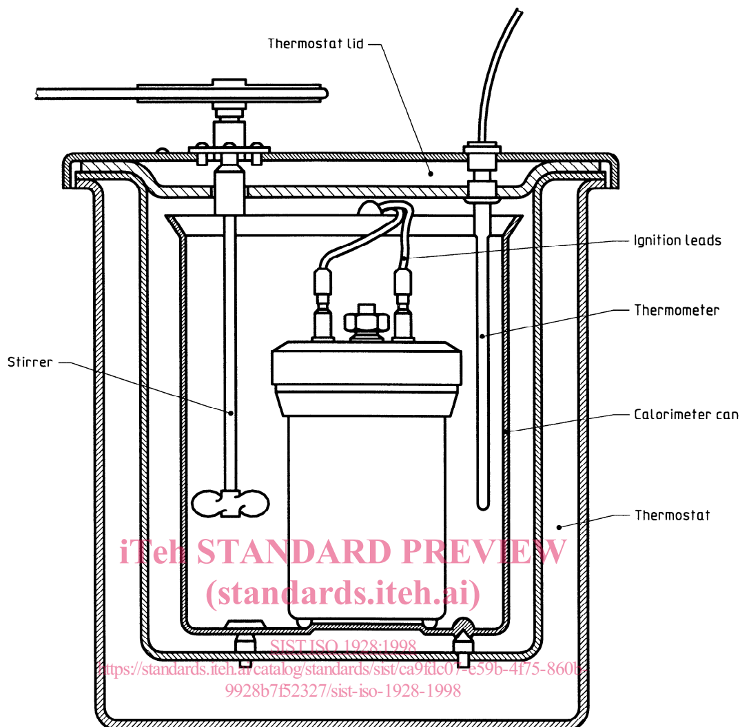
Figure 1 — Classical-type bomb combustion calorimeter with thermostat
