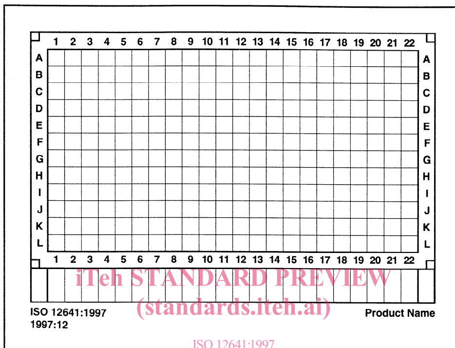
ISO 12641:1997 https://standards.iteh.ai/catalog/standards/sist/24327e85-a975-4342-b9bf-1b496c3d8e10/iso-12641-1997 Figure 1 — Layout, Type 1 colour transmission target
