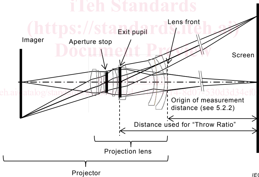
Figure 1 – Exit pupil in projector
