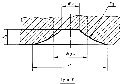
Figure 4 — Lubrication pocket
