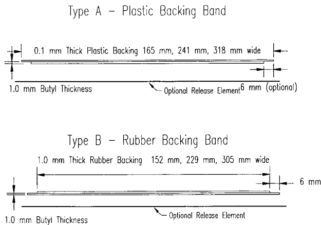
FIG. 3 Sealing Band Type III (Not to Scale)
