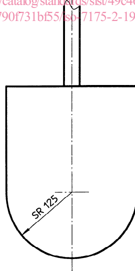
Figure 2 — Bottom impactor
