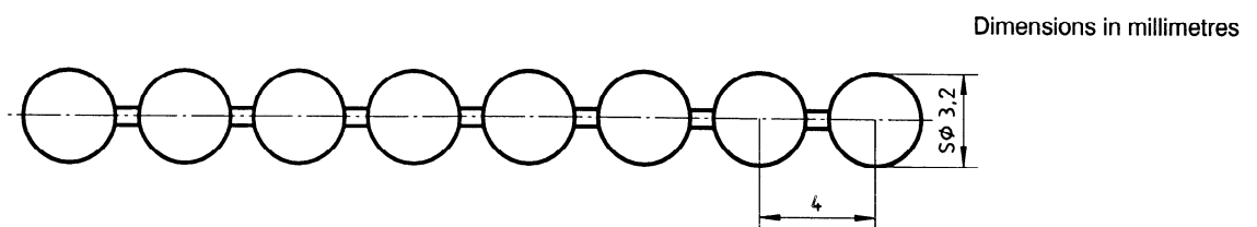
Figure 4 — Ball chain
