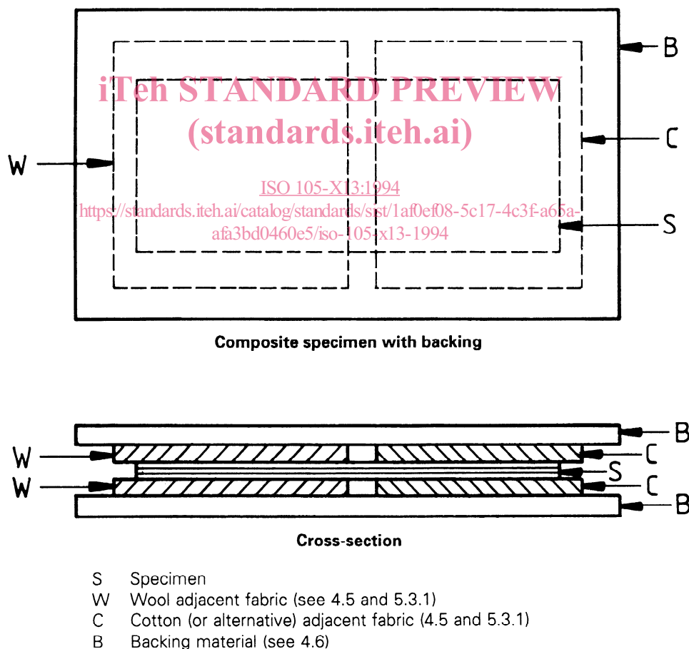
Figure 1 — Composite specimen
