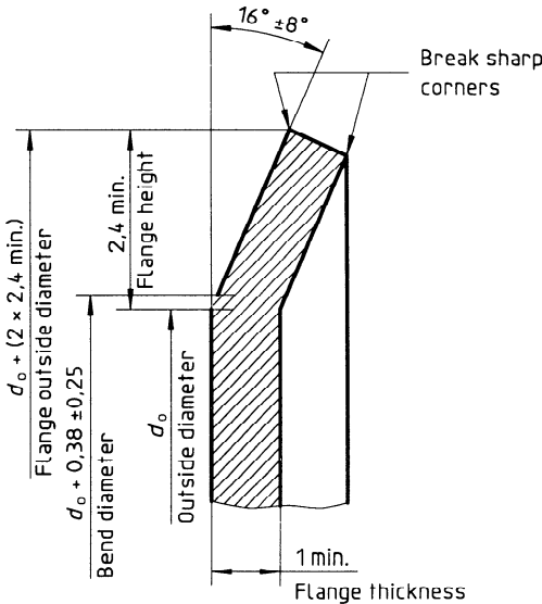
Figure 8 — Flange dimensions
