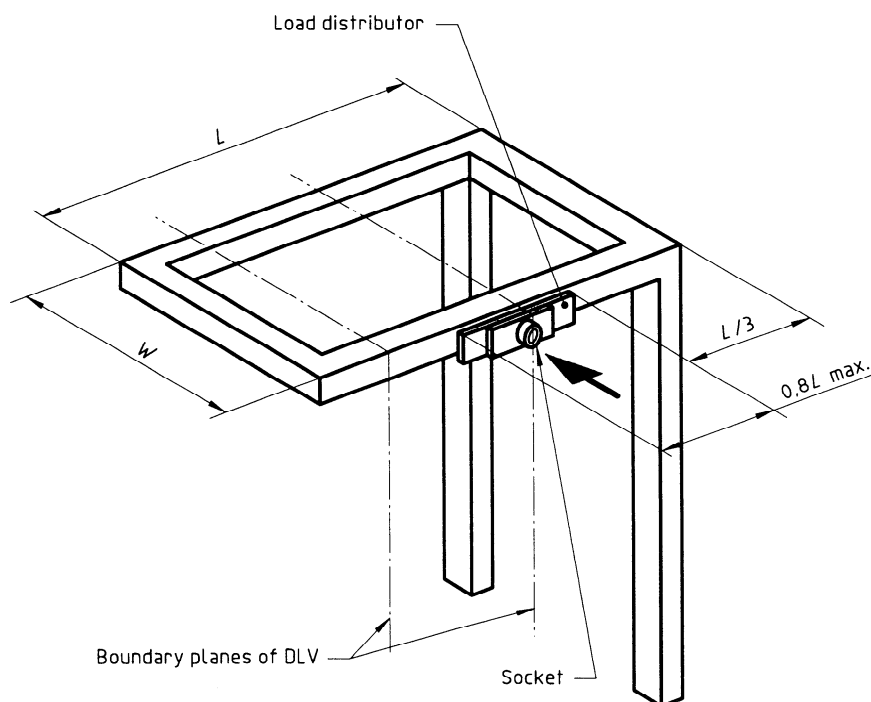
Figure 2 — Two-post TOPS lateral load application point (standards.iteh.ai)
