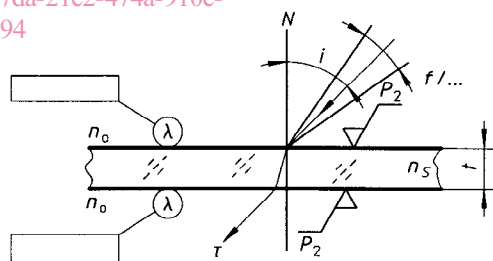
Figure A.4 — Transmittance, incidence oblique, conique
