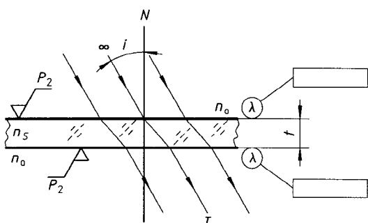
Figure A.2 — Transmittance, faisceau collimaté
