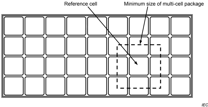
Figure 2 – Single reference cell in a multi-cell package
