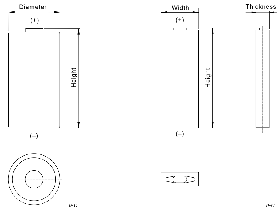
Figure 1 – Jacketed cylindrical cells Figure 2 – Jacketed small prismatic cells
