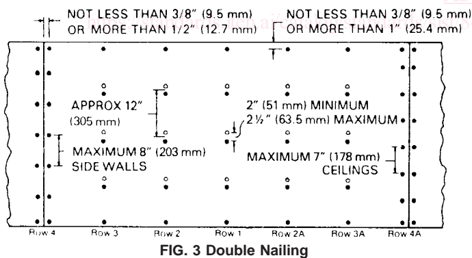
FIG. 3 Double Nailing
