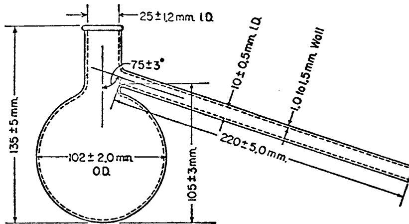
FIG. 1 Distillation Flask
