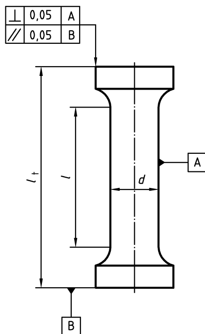
Figure 1 - Type 1 specimen geometry
