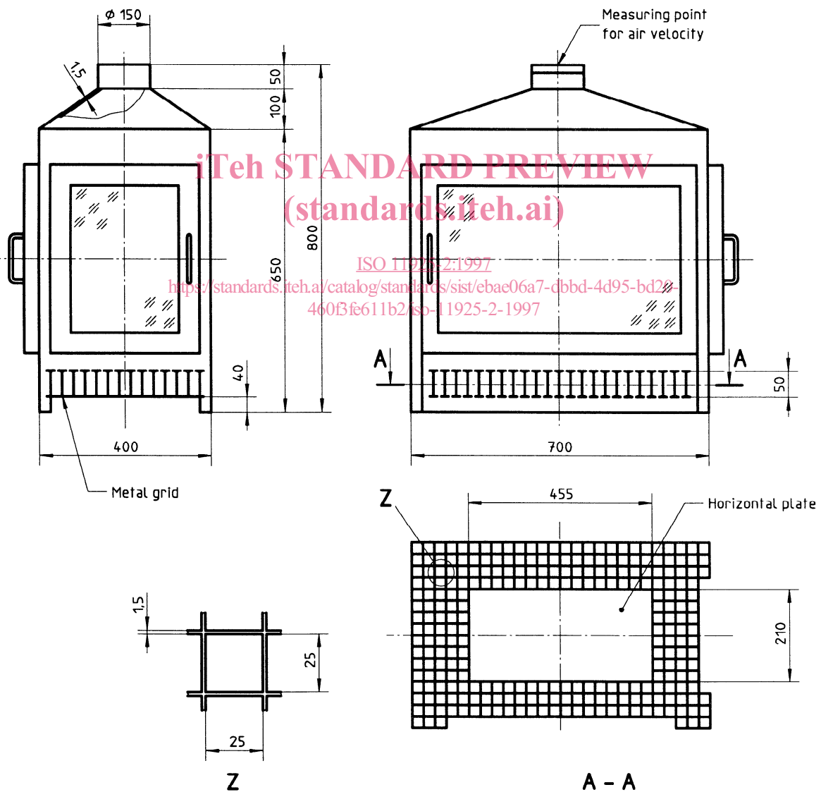
Figure 1 — Combustion chamber
