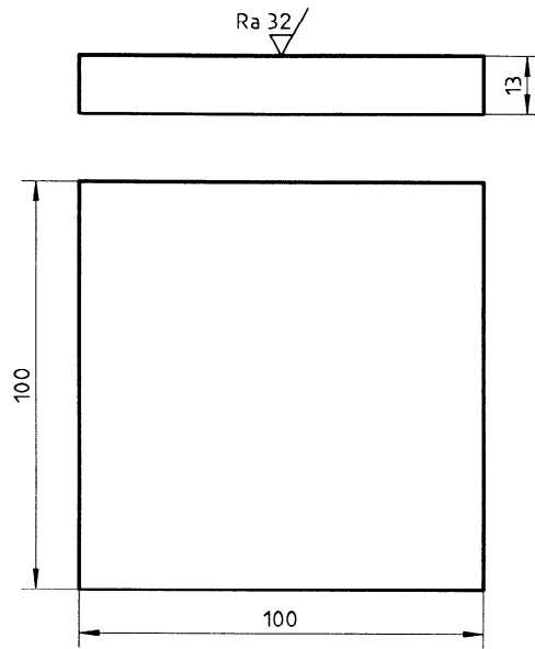
Figure 1 — Base plate
