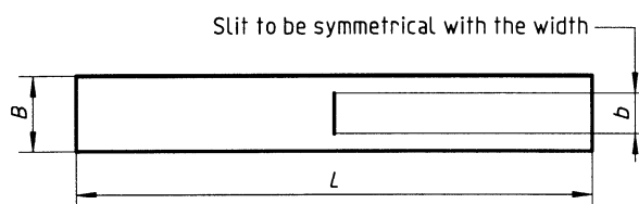
Dimensions of test piece
