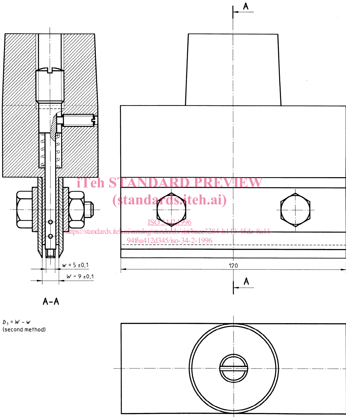
Figure 1 — Die for Delft test pieces
