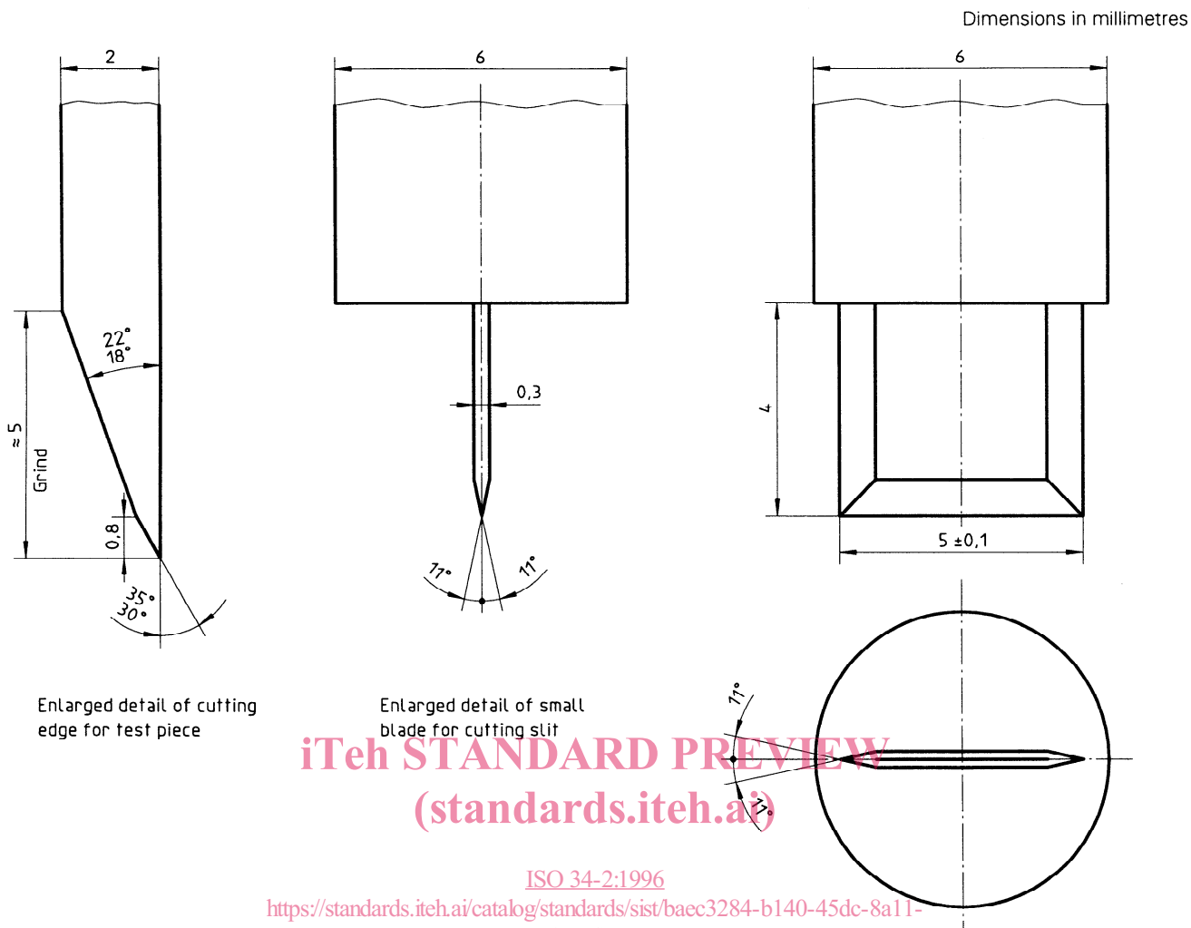
Figure 2 — Details of Delft test piece die cutting edges
