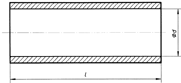
Figure 1 — Tube cylindrique
