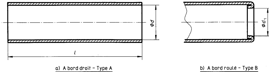
Figure 1 — Tubes cylindriques
