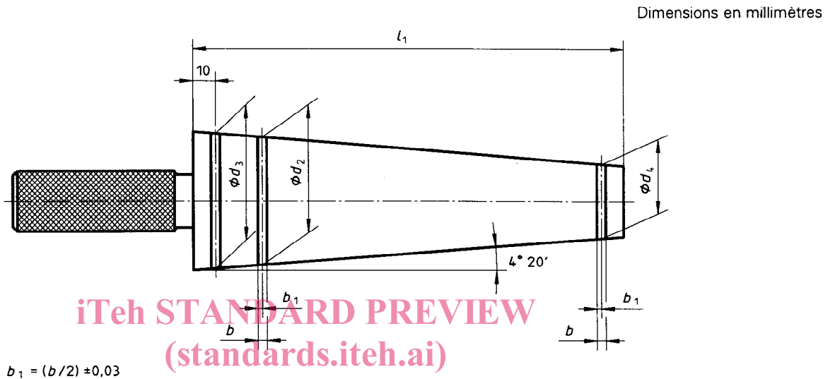
ISO 8489-4:1995 Figure 2 — Calibre https://standards.iteh.ai/catalog/standards/sist/6629c99b-41dc-4440-adee-1e59a7982cd6/iso-8489-4-1995
