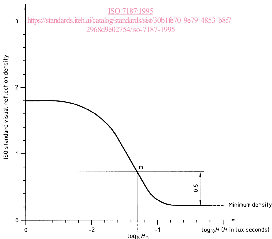
Figure 1 — Sensitometric curve
