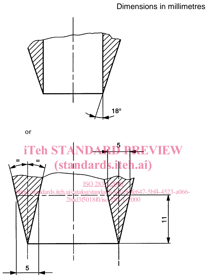
Figure 2 - Suitable die profiles
