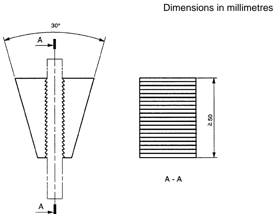
Figure 1 - Grip with transverse serrations
