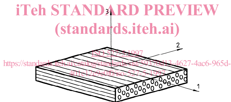
Figure 2 — Unidirectionally reinforced plastic composite showing axes of symmetry
