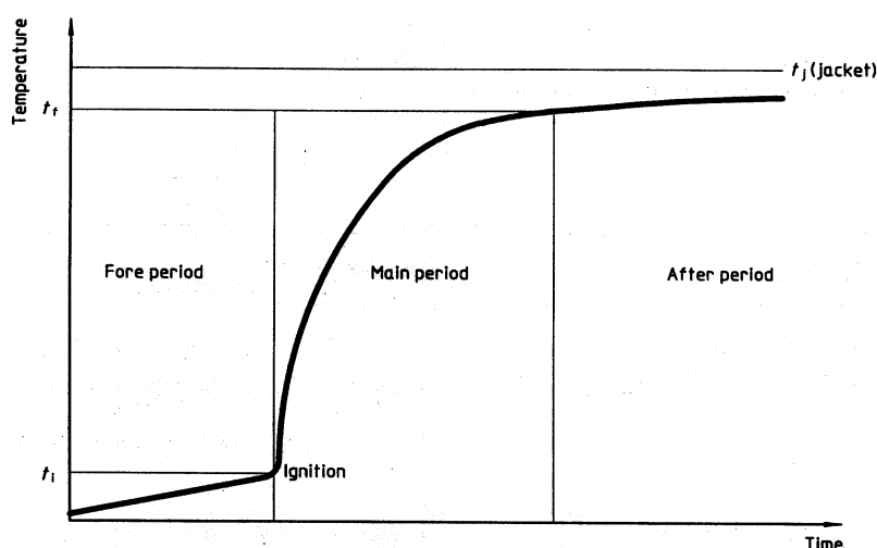
Figure 2 - Time-temperature curve (isoperibol calorimeter)
