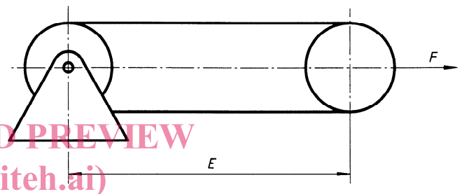
Figure 1 — Measuring device
