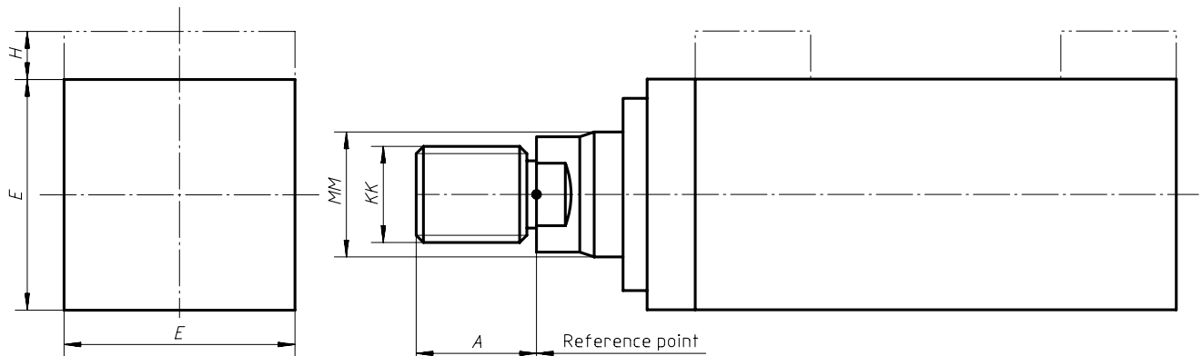
Figure 1 — Basic dimensions (standards.iteh.ai)
