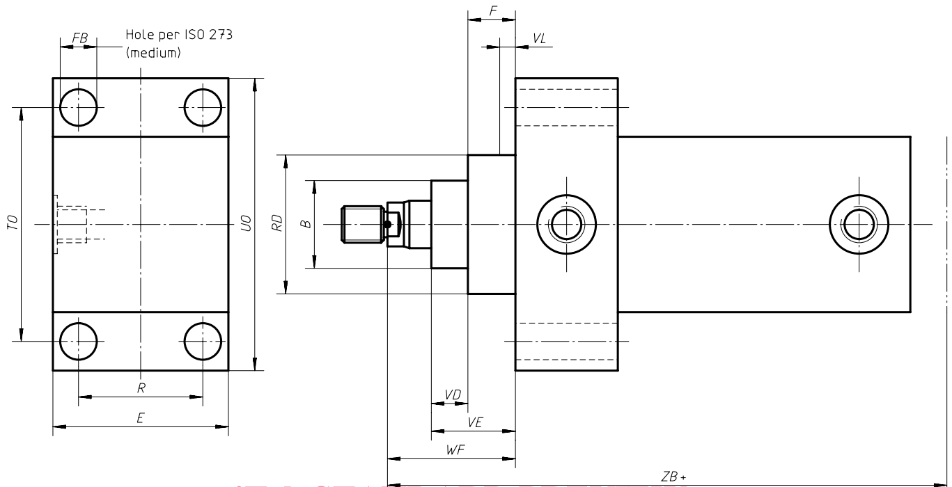
Figure 3 — ME5 — Rectangular flange, integral with head (standards.iteh.ai)
