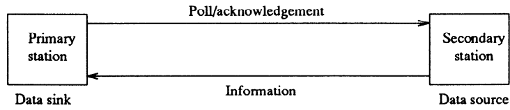
Figure 2 — Unbalanced data link configuration (case 2)
