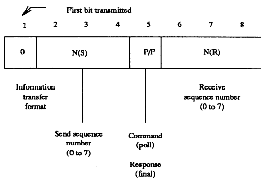
Figure 4 - Information transfer format of control field bits
