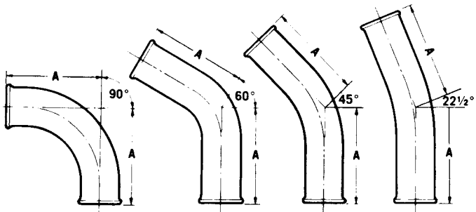
¼ bend (90°) ¼ bend (60°) ⅓ bend (45°) ⅓ bend (22½°) A Dimensions A , in.
