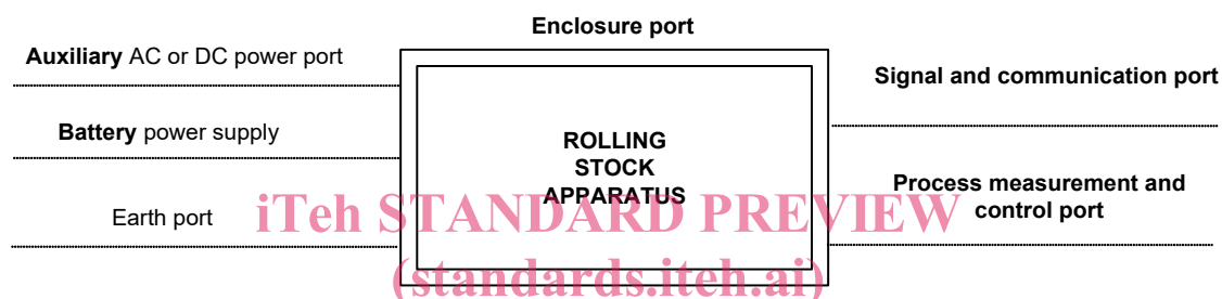
IEC 62236-3-2:2018 Figure 1 – Main categories of ports https://standards.iteh.ai/catalog/standards/sist/b0c6d8c1-91c6-45ac-b437-3b181720ac82/iec-62236-3-2-2018
