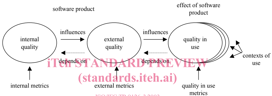
ISO/IEC TR 9126-3:2003 https://standards.iteh.ai/catalog/standards/sist/a0f913a0-1ac9-4b4f-a306-a271d122dc59/iso-iec-tr-9126-3-2003 Figure 1 – Relationship between types of metrics
