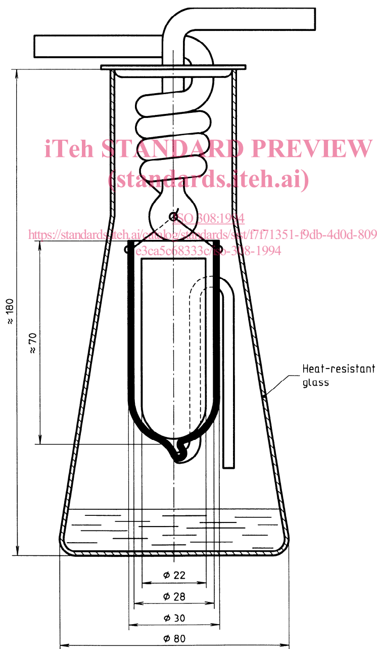
Figure 1 — Extraction apparatus
