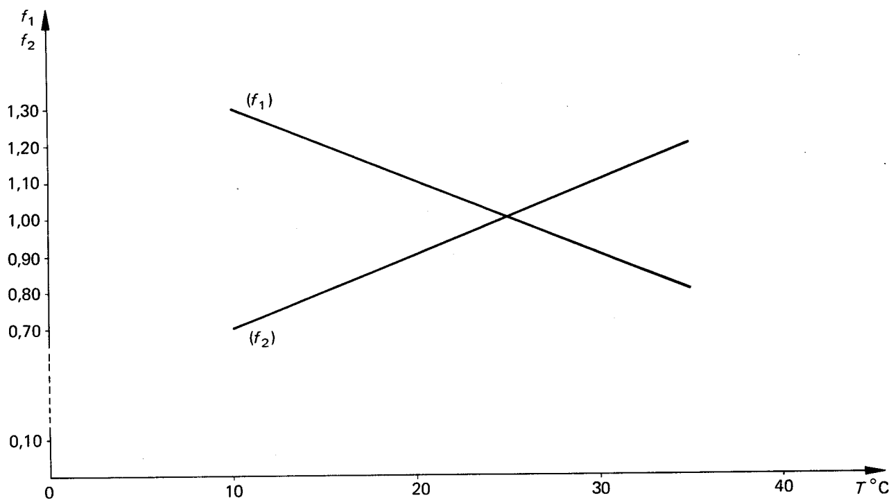
FIGURE — Variation of coefficients f_1 and f_2 as a function of temperature (in °C)
