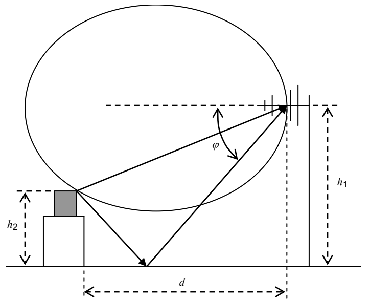
Figure 1 – Schematic of radiation from EUT reaching an LPDA antenna directly and via ground reflections on a 3 m site, showing the half beamwidth, \varphi , at the reflected ray
